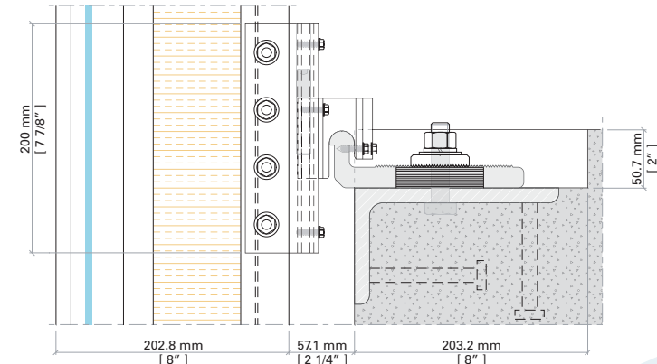
Fully Capped Expansion Joint / Aluminum Panel
