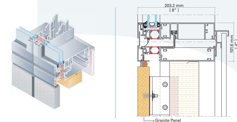
Fully Capped Expansion Joint / Granite Panel
